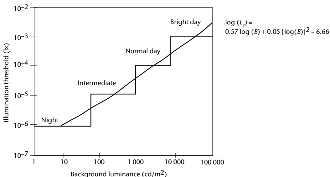
Figure D-1. Relationship between the illumination threshold E_T (lx) and background luminance B ( \text{cd}/\text{m}^2 )
